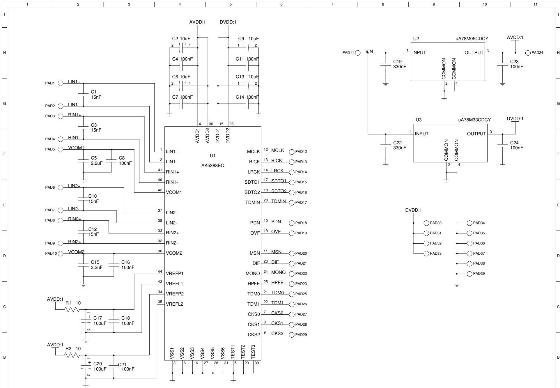
AK5388 Breakout Board Schematic. Copyright © 2011 by Stephen C. Trier.
